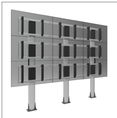
Solution 2: VideoWall system including, small base plate fastened to floor
