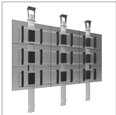
Solution 4: VideoWall system including small floor and ceiling plate, to fasten in between floor and ceiling
